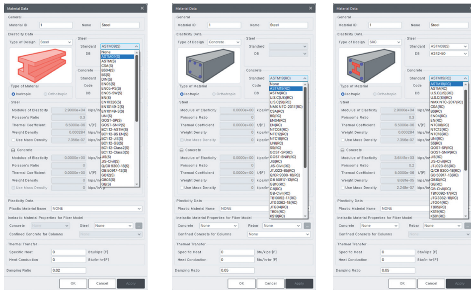
Concrete/Steel/Composite Materials
