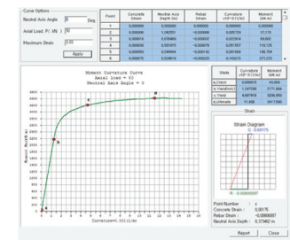
Moment-Curvature Curve
